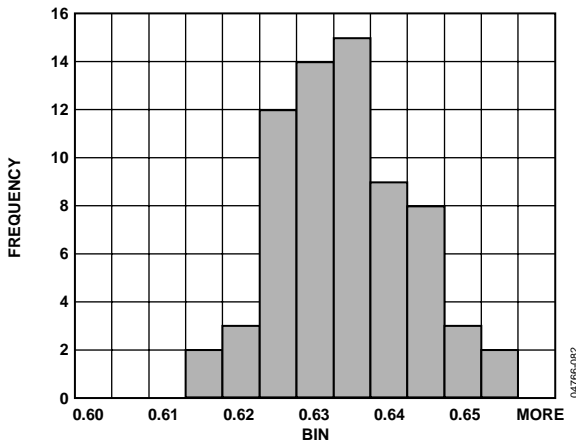
Figure 24. I_{DD} Histogram @ V_{DD} = 5V
