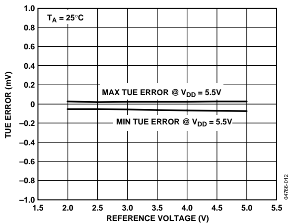
Figure 12. TUE vs. Reference Input Voltage
