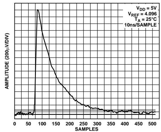
Figure 21. Glitch Energy
