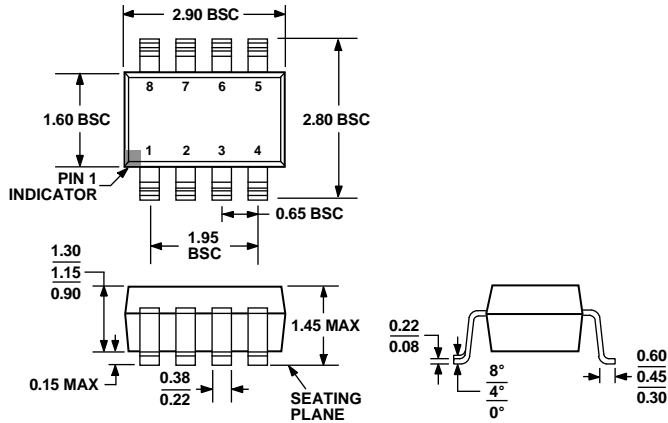
Figure 45. 8-Lead Small Outline Transistor Package [SOT-23] (RJ-8)
